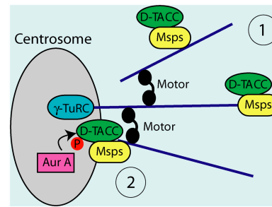
Figure 7. A schematic model of how the D-TACC-Msp complex stabilizes MTs in D. melanogaster embryos. MTs are nucleated at centrosomes by the \gamma -tubulin ring complex ( \gamma -TuRC). These MTs are often released from \gamma -TuRC but are held in the vicinity of the centrosome by the action of MT motors. The bulk of D-TACC-Msp complexes (that are present at centrosomes, along MTs, and throughout the cytoplasm) can bind these MTs either laterally or at plus ends and stabilize them (mechanism 1). Aurora A can specifically activate a small fraction of D-TACC-Msp complexes that are at the centrosome. This allows the phosphorylated complexes (P, red) to interact with and stabilize MT minus ends (mechanism 2). Importantly, this mechanism is only active at centrosomes, and any MTs that form in the cytoplasm will not be stabilized in this way. This may explain, at least in part, why centrosomes are such dominant sites of MT assembly in mitosis.
